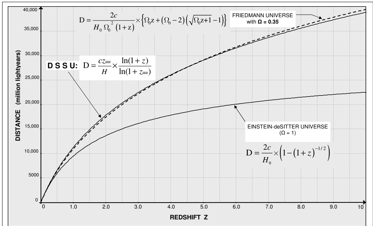
Graph 2. Redshift-Distance relation for redshifts between 0 and 10. The parameters used in the equations are: the redshift across one cosmic cell z_{CC} = 0.01823 , the space-expansion term H and the Hubble term H_0 are both 18.5 km/s /Mly, the density ratio \Omega as shown, and the
