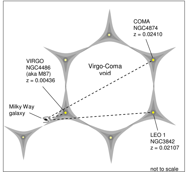
Fig. 3. Determining the redshift across a cosmic cell. The difference in the z values between M87 and NGC4874 is 0.01974; the difference between M87 and NGC3842 is 0.01671. The average difference is 0.01823. The redshift across a typical cosmic cell is symbolized by z_{CC} and assigned the empirical value 0.01823. (The hexagonal unit in this schematic drawing represents a polyhedral cosmic cell. Size of galaxies is greatly exaggerated.)
