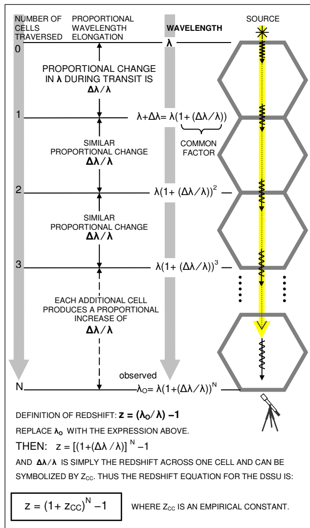
Fig. 2. Cosmic-redshift equation for the DSSU is unique for a universe with vacuum expanding within a static structure. Starting at the top of the diagram, each cosmic cell (cc) contributes a redshift component to a quantum of radiation. Each progressively altered wavelength is the previous one plus its proportional change, hence the common factor (1 + (\Delta\lambda/\lambda)) .
