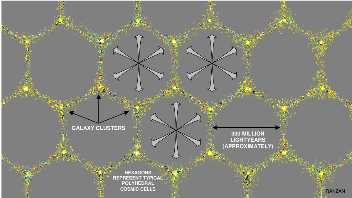
Fig. 1. The Dynamic Steady State Universe consists of the simultaneous, but spatially-separated, expansion and contraction of the space medium. These balanced dynamic processes produce a more or less static polyhedral pattern. According to DSSU theory and astronomical observations, our Universe is cellularly structured (shown here idealized). Although the vacuum expands in the interior (the void) of the cells, the cells themselves do not increase in size . At the boundaries of the cells, where gravity dominates, the space medium is contracting. The cells maintain equilibrium; consequently the universe does not expand .
