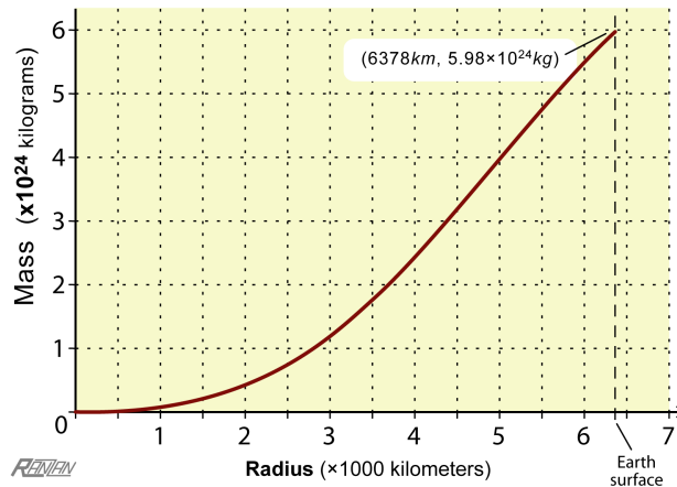
Figure 8. Graph of Earth's interior-mass function. The function gives the total mass inside a radius specified by the variable r . Notice that the distance corresponding to the Earth's surface gives an ordinate that agrees with the official whole-Earth mass value of 5.98 \times 10^{24} \text{ kg} ; and thus, serves as a check on the general correctness of the density function.
