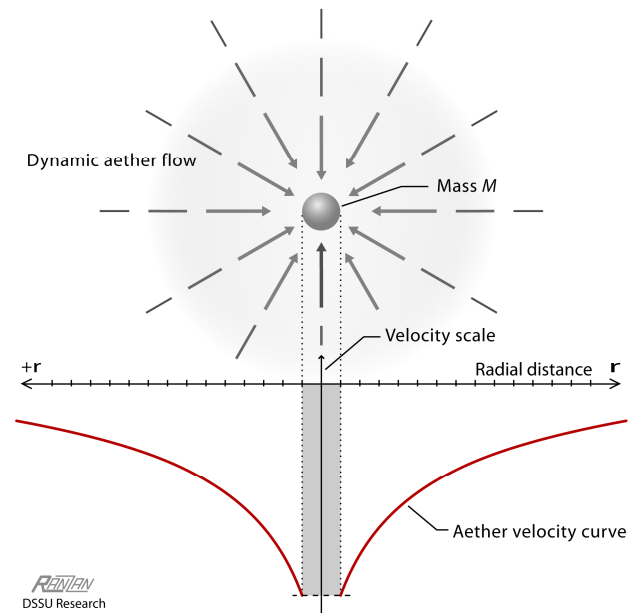
Fig. 1. Schematic of the gravity well (top) shows the flow of aether into the central mass. The flow is an accelerating stream that nominally models Newtonian gravity. Just below is the graph representing the velocity of the flow of the space medium in accordance with the equation given in the text.
