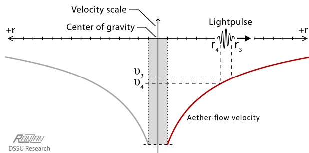
Fig. 3. Lightpulse ascending a gravity well "experiences" a flow differential between its front and back ends (whose instantaneous positions from the center of gravity are r_3 and r_4 , respectively). As a consequence, the pulse undergoes elongation and acquires a spectral redshift—a velocity differential redshift. (Pulse is greatly exaggerated in size.)
