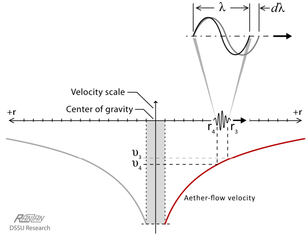
Fig. 5. Lightwave elongation during outbound propagation through the gravity well. The wave/photon is being conducted by aether whose speed of inflow accelerates with proximity to the gravitating structure. As a result, the photon’s front and back ends “experience” a flow differential. The wavelength increases during the ascent within the gravity well, shown here by its aether-flow velocity curve.
