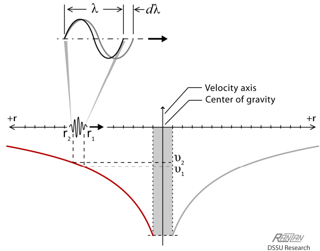
Fig. 4. Lightwave elongation during inbound propagation through the gravity well. The wave/photon is being conducted by a space medium whose speed of inflow increases with proximity to the gravitating structure. As a result, the photon's front and back ends "experience" a flow differential. The wavelength increases during the descent into the gravity well, which is shown here by its aether-flow velocity curve. (The radius axis is positive in both directions by virtue of using a cylindrical coordinate system.)
