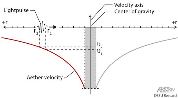
Fig. 2. Lightpulse entering a gravity well "experiences" a flow differential between its front and back ends. As a consequence, the pulse tends to elongate; the pulse undergoes an elementary redshift process. (Note, the use of a cylindrical coordinate system, making the radius axis positive in both directions.)
