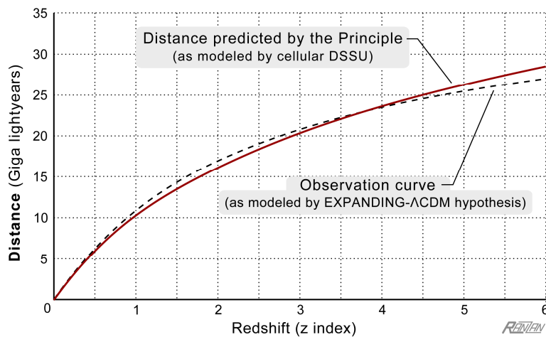
Fig. 7. Cosmic redshift is interpreted in accordance with the Principle of velocity differential propagation (solid curve). The dashed curve represents the cosmic-redshift-versus-cosmic-distance relationship based on astronomical observations over many decades using sophisticated techniques. The “prediction” curve agrees remarkably well with the “observation” curve. Note that the observation curve is modeled by the expanding- \Lambda CDM hypothesis; reasonable agreement is obtained by adjusting its various parameters none of which has a connection to physical reality.
