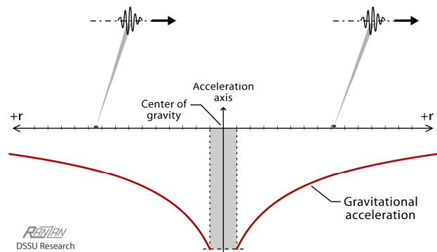
Fig. 6. Light pulse transiting a gravity well. During the descent, the gravitational acceleration acting on the leading end of the pulse is slightly more intense than the acceleration on the trailing end. This differential in the acceleration manifests as an intrinsic elongation. During the ascent, the situation is reversed; the gravitational acceleration acting on the fore end is slightly less intense than what is experienced by the back end. In other words, the trailing end is being "dragged back" more than is the front end. Consequently, there is again an intrinsic stretch. (Gravitational acceleration: a = -GM/r^2 ) (Note again, the use of a cylindrical coordinate system.)
