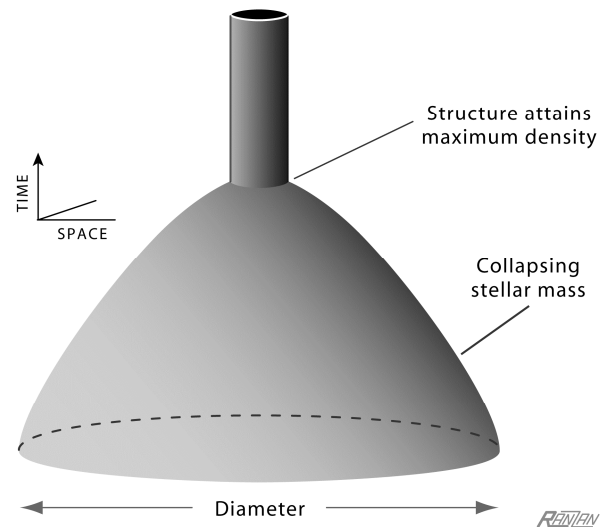
Figure 1. Gravitational collapse halts when mass concentration attains the ultimate density. Based on (1) the existence of aether, as was defined; (2) the innate absorption/consumption of aether by all matter; (3) the reasonable assumption of the existence of a density limit; and (4) the concentration or aggregation of sufficient degenerate mass having complete absence of thermal agitation; based on those factors, nature follows a course that ultimately leads to a final stage of gravitational collapse (shown in the schematic). The end result is a compact-and-stable structure with maximal density.
