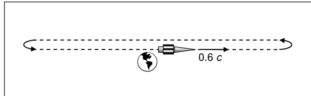
Fig. 5. Since constant-speed linear motion is a form of absolute motion, clock slowing is to be expected; hence, no twin paradox . (The paradox is confined to ESR.) The space journeys, instead of being circular as in Fig. 2 , are straight-out and straight-back trips repeated over and over. Acceleration plays a momentary but otherwise negligible part. Practically all the clock slowing occurs during inertial motion.
