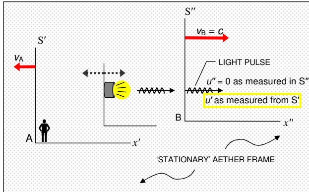
Fig. 7. The speed of light is constant through aether — and the relative speed of light appears constant for all observers. The velocity v_A of the observer and the velocity v_B of the light pulses are absolute velocities with respect to the aether medium . Motion of the light source does not, in any way, affect the speed of the light pulses through aether. Light pulses (or waves) are conducted by the aether at a constant rate of c \approx 300,000 km/s. Observer A measures the velocity of the light pulse as ( u' ) —as predicted in the text, its value is always c .
